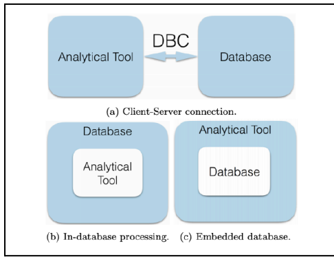
Figure 2.1 In-Database Theory (Amevor, 2020)
